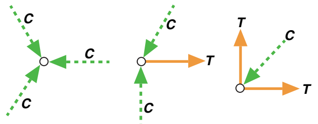
Fig. R23.2.6b—Extended nodal zone showing the effect of the distribution of the force.
