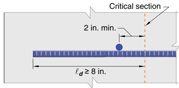
Fig. R25.4.6.3—Development of welded deformed wire reinforcement.
