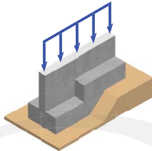
Stepped footing
