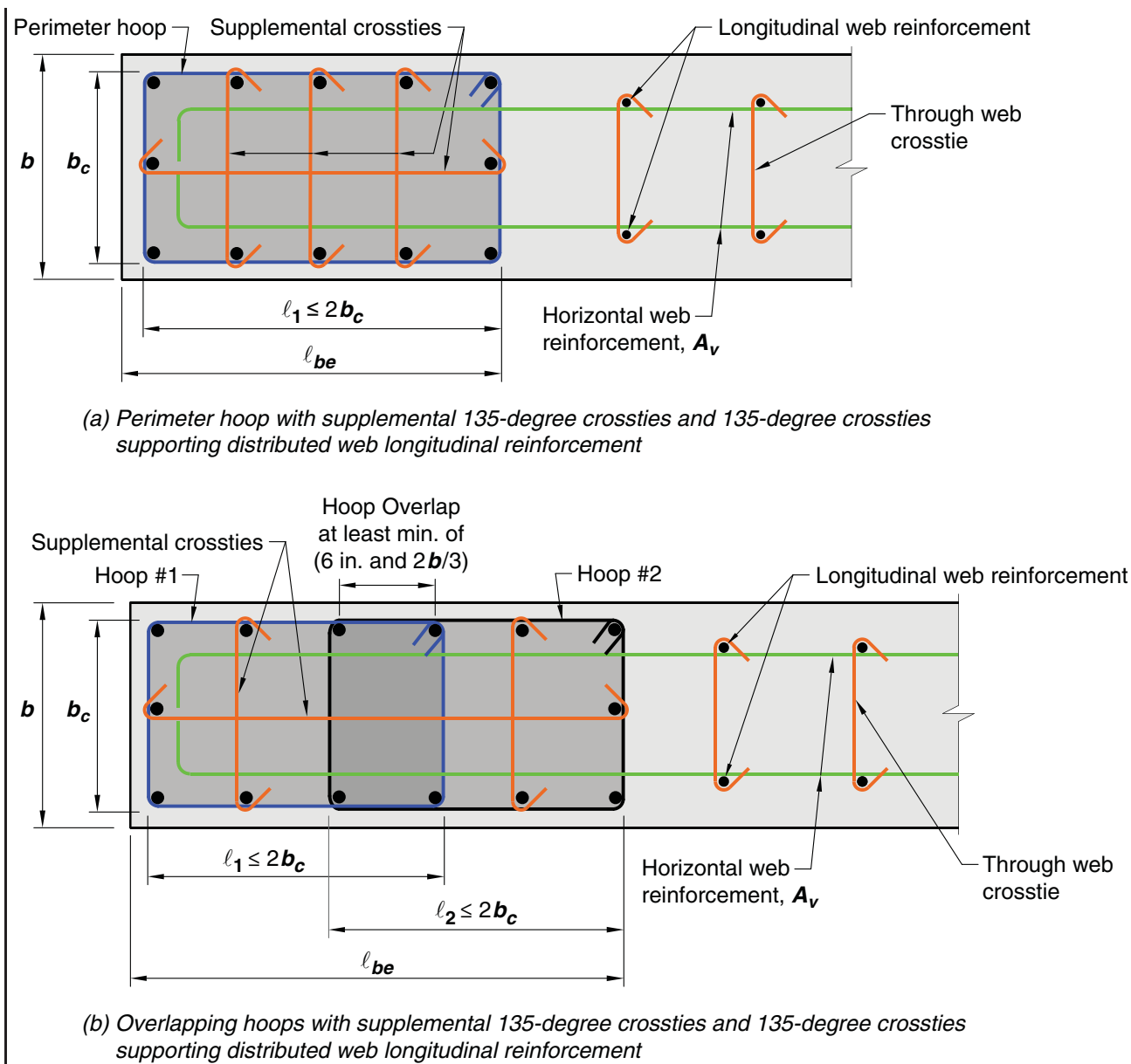
Fig. R18.10.6.4a—Configurations of boundary transverse reinforcement and web crossties.
