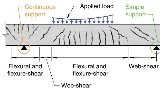
Fig. R22.5.6.3—Types of cracking in concrete beams.
