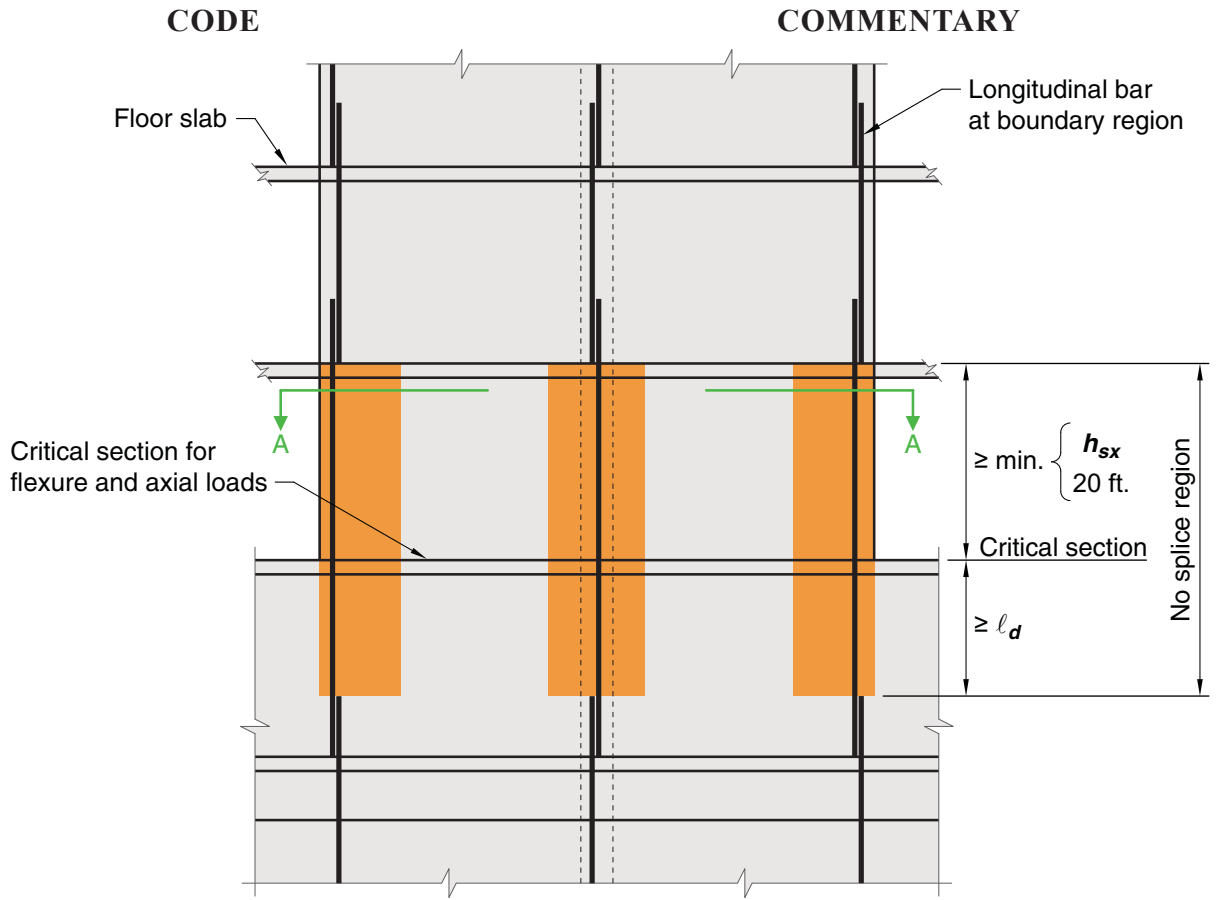
(a) Elevation
