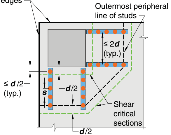
Fig. R8.7.7—Typical arrangements of headed shear stud reinforcement and critical sections.
