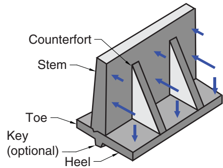
Counterfort/butressed
