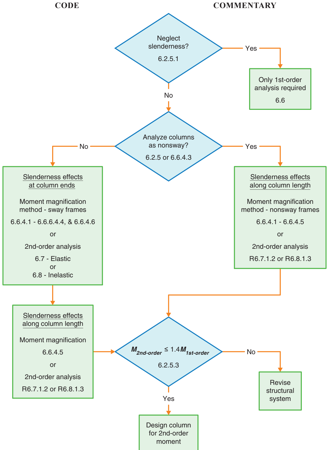
Fig. R6.2.5.3—Flowchart for determining column slenderness effects.
