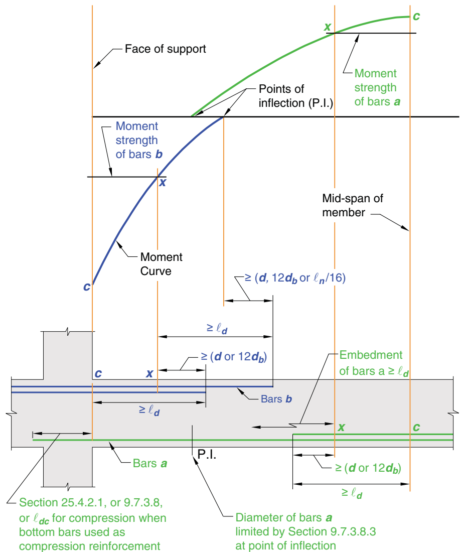
Fig. R9.7.3.2—Development of flexural reinforcement in a typical continuous beam.
