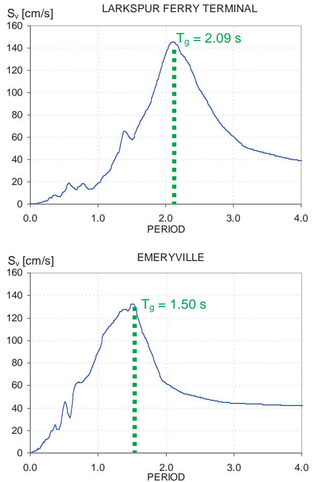
Figure 3-15 Predominant ground motion periods for the soft soil records obtained at Larkspur Ferry Terminal and Emeryville during the 1989 Loma Prieta earthquake.
