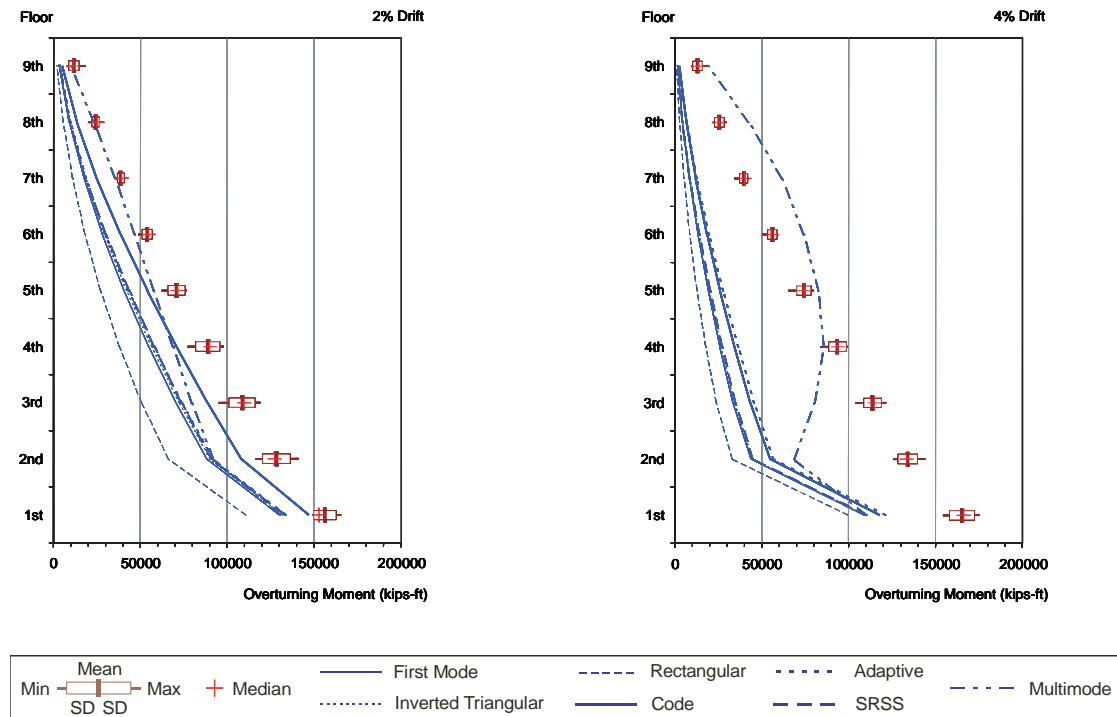
Figure 10-4 Overturning moments in example 9-story building using various load vectors.
