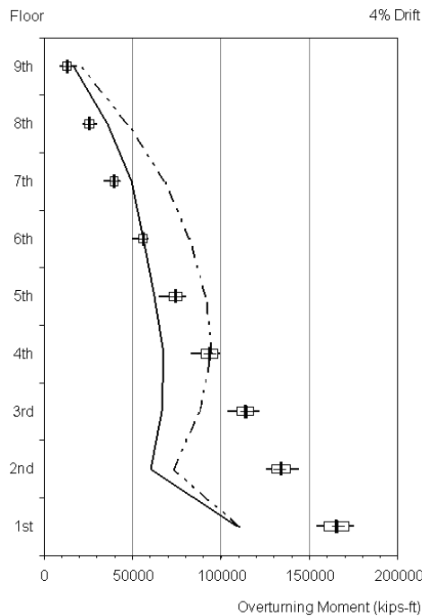
(f) Overturning moments for 9-story weak story frame at 4% drift
