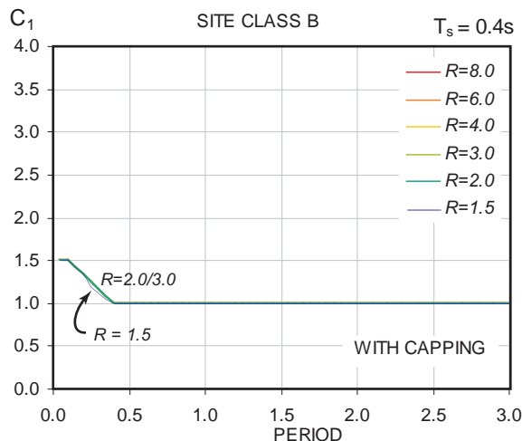
Figure 3-13 Comparison between the mean C_1 computed from nonlinear response-history analyses to C_1 in FEMA 356 (non-capped and capped).
