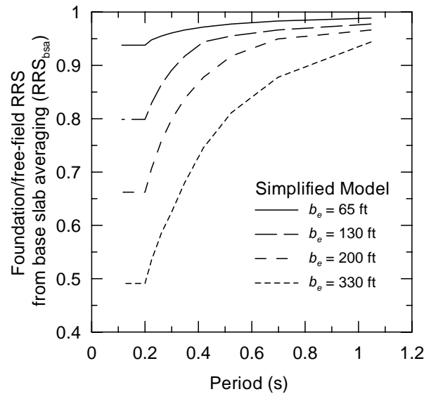
Figure E-6 RRS from simplified model as function of foundation size, b_e
