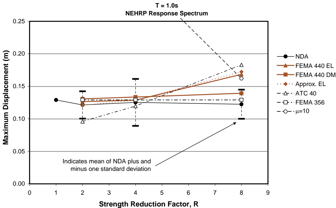
Figure 7-10 Comparison of responses for an oscillator with T = 1.0 s calculated using various procedures, response spectra scaled to the NEHRP spectrum, and values calculated for the NEHRP spectrum.
