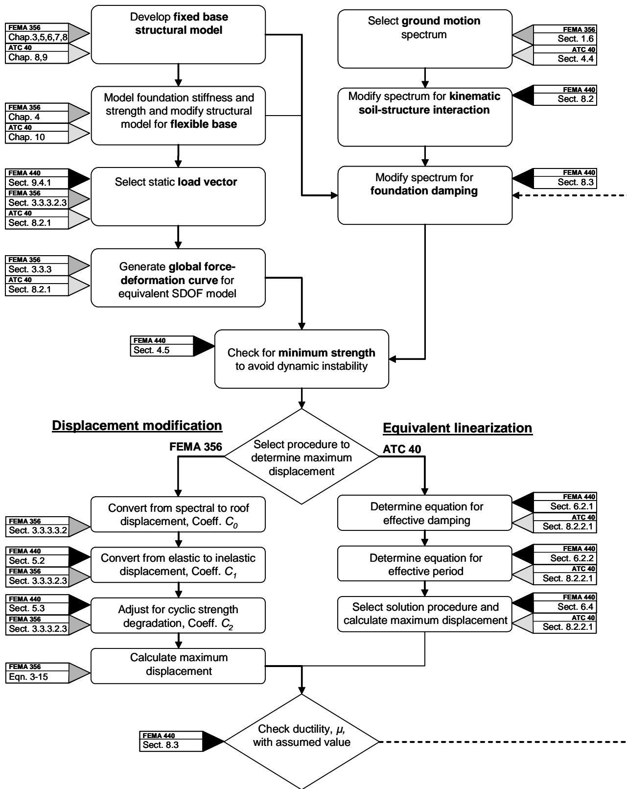
Figure 10-7 Application flowchart for nonlinear static seismic analysis
