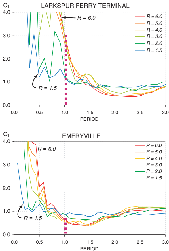
Figure 3-14 Variation of C_1 for two individual ground motions recorded on soft soil E.
