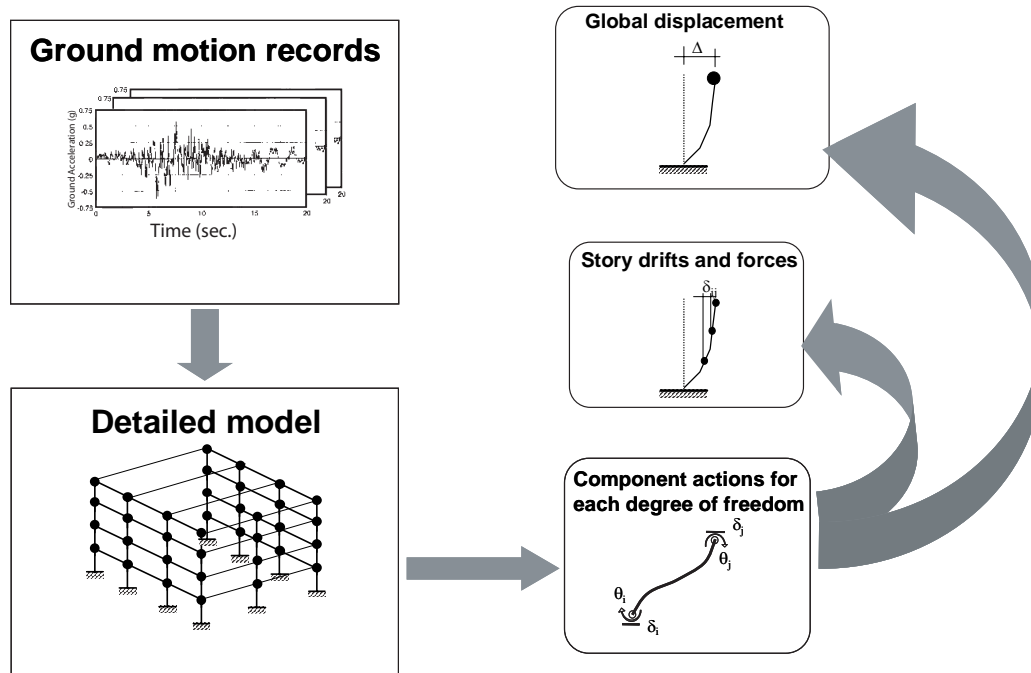
Figure 2-7 Flow chart depicting the nonlinear dynamic analysis process. Note that component actions are used to determine higher-level effects, such as story drifts and roof displacement, \Delta .
