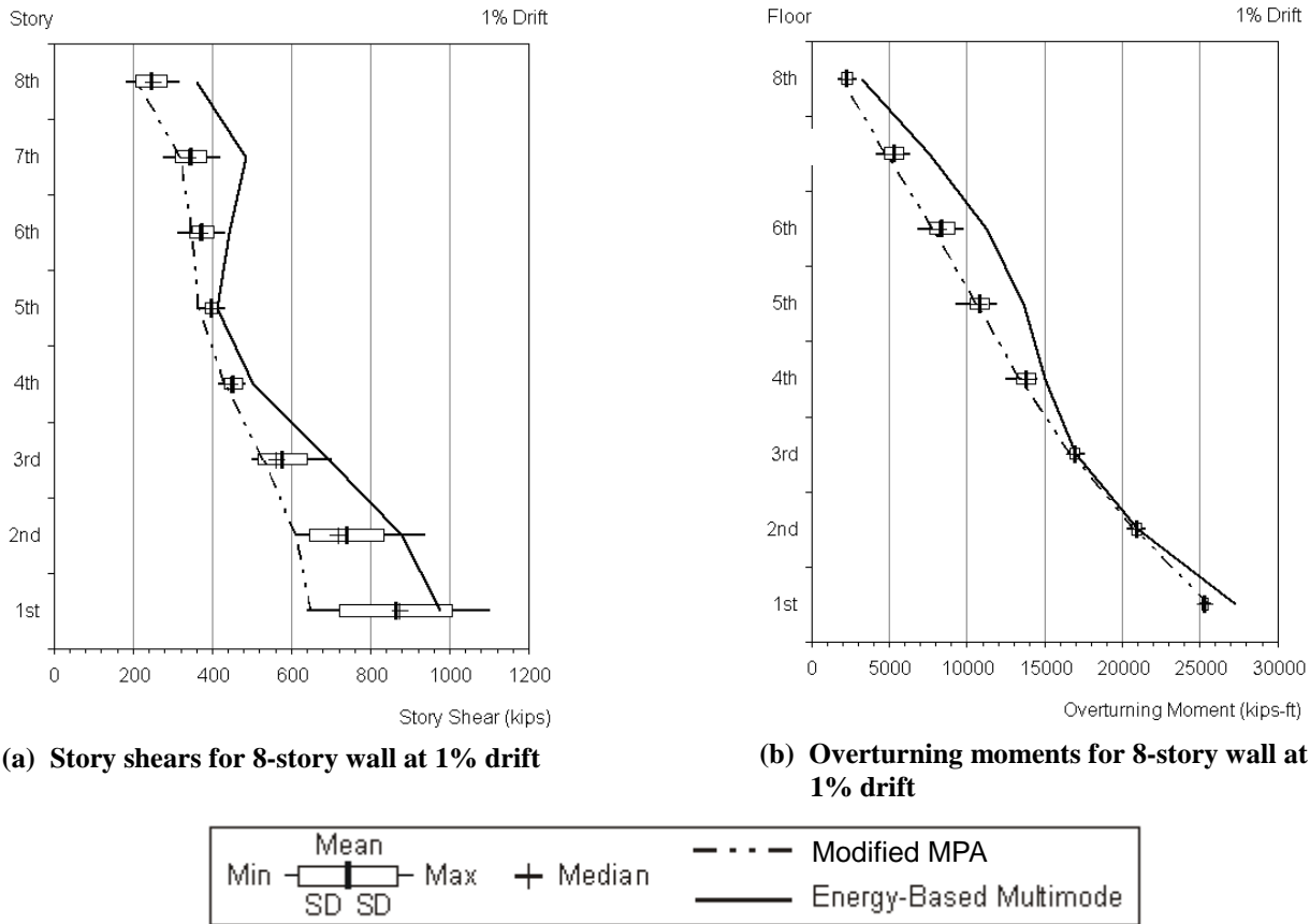
Figure F-16 Example comparisons of energy-based and conventional multiple mode calculations.
