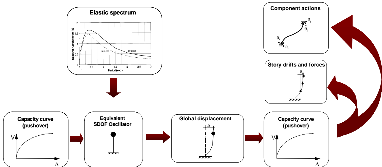
Figure 2-10 Flow chart depicting the process followed in nonlinear static procedures. Note that component actions are based on global displacement demand and a pushover/capacity curve.
