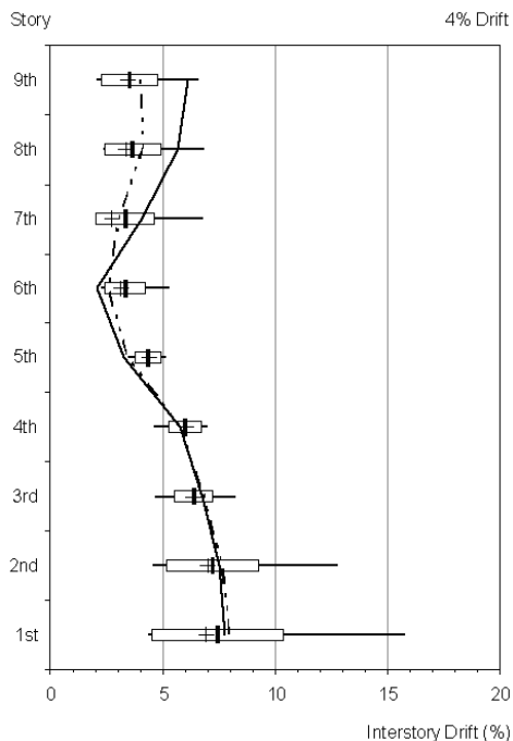
(c) Interstory drifts for 9-story frame at 4% drift
