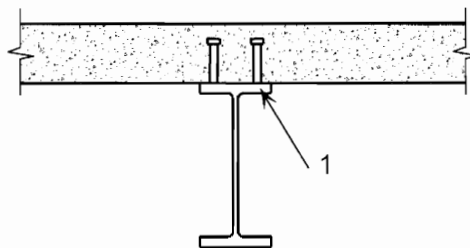
1 compression flange
