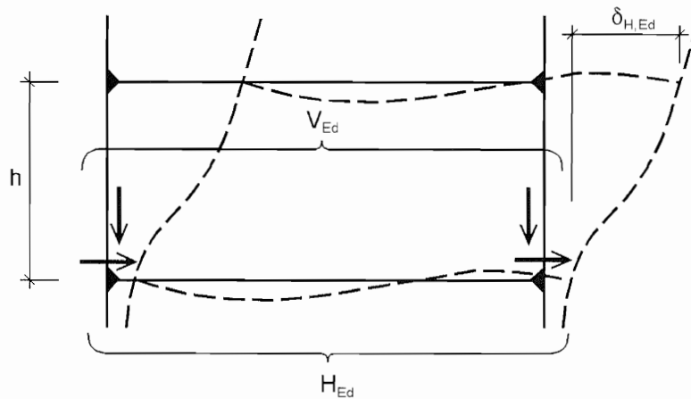
AC2 Figure 5.1: Notations for 5.2.1(4) AC2
