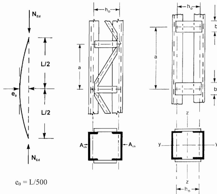
Figure 6.7: Uniform built-up columns with lacings and \langle AC_2 \rangle battens \langle AC_2 \rangle
