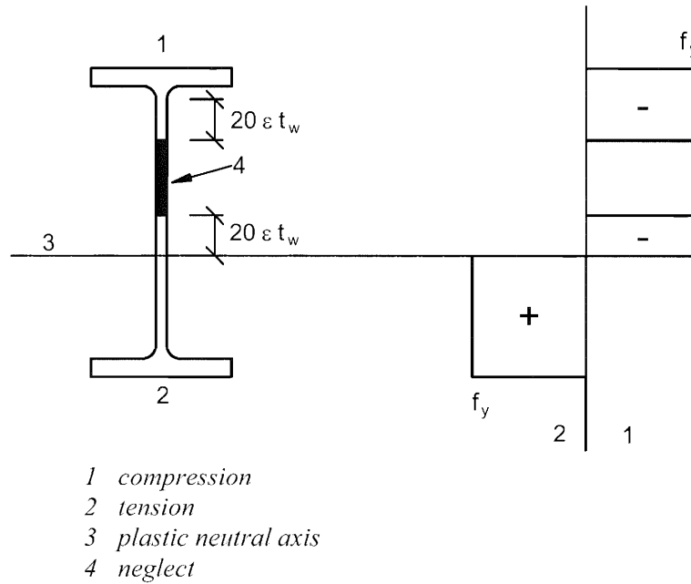
Figure 6.3: Effective class 2 web
