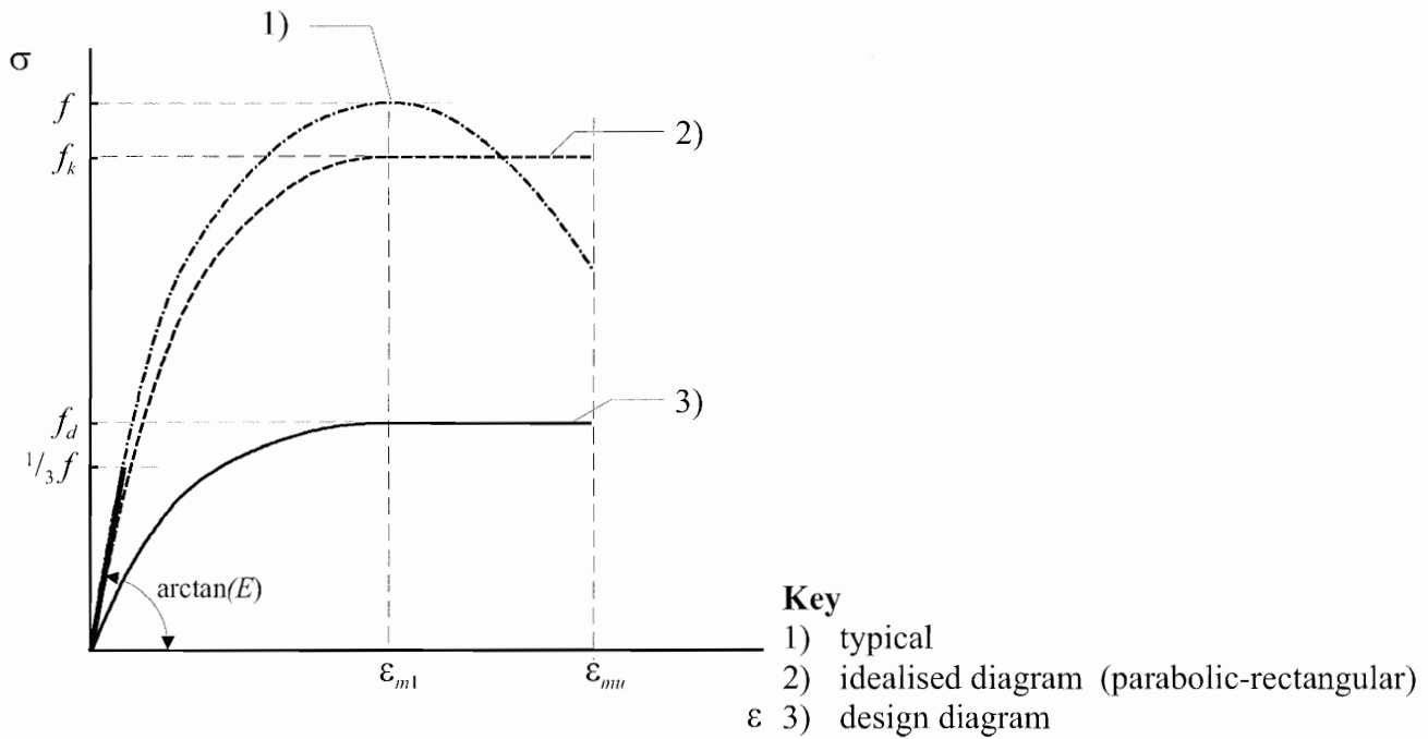
Figure 3.2 — Stress-strain relationship for masonry in compression
