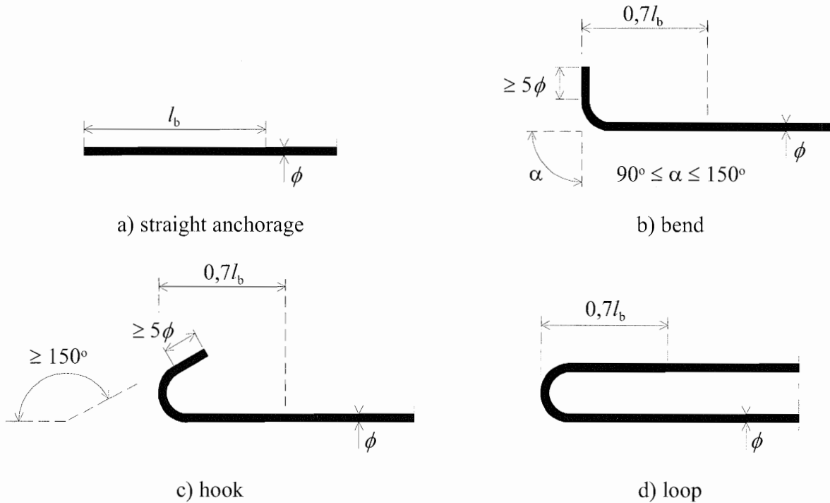
Figure 8.3 — Anchorage details
