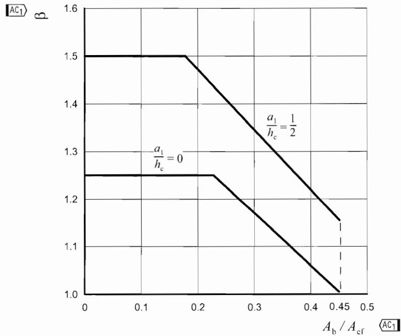
Figure H.1 — Graph showing the enhancement factor as given in 6.1.3: Concentrated loads under bearings
