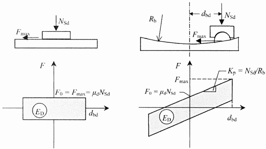
Figure 7.3: Friction force-displacement behaviour
