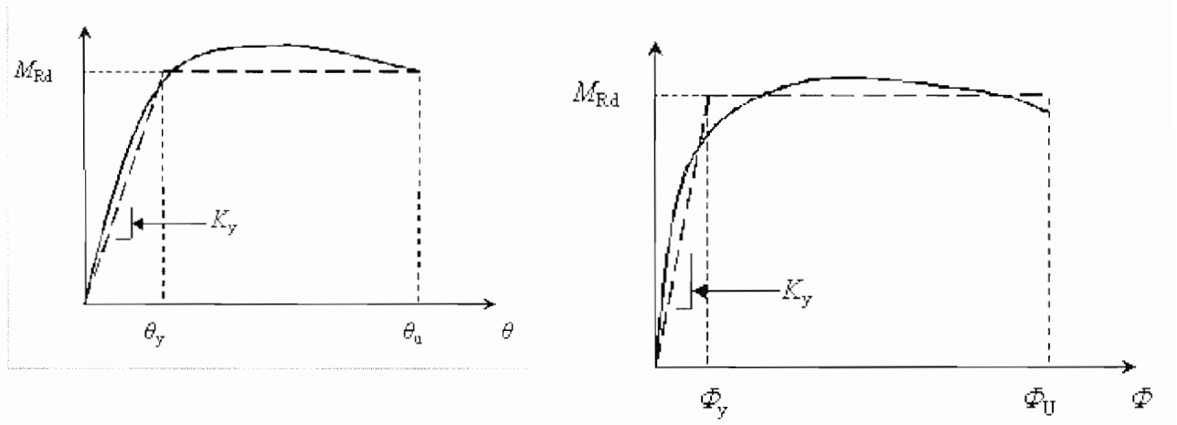
Figure 2.5: Moment - deformation diagrams at plastic hinges
